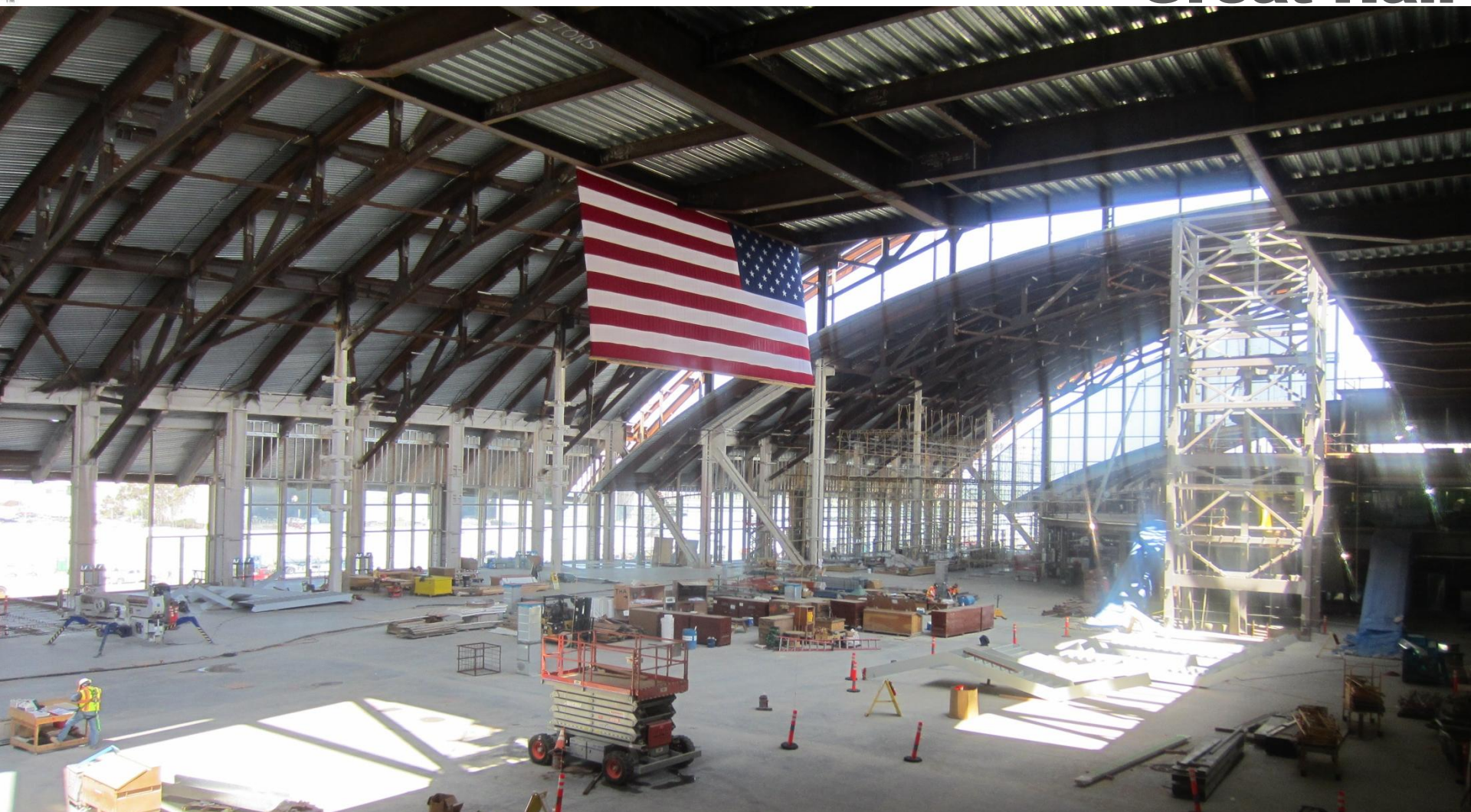
Interior of the Great Hall looking northwest. May 17, 2012
