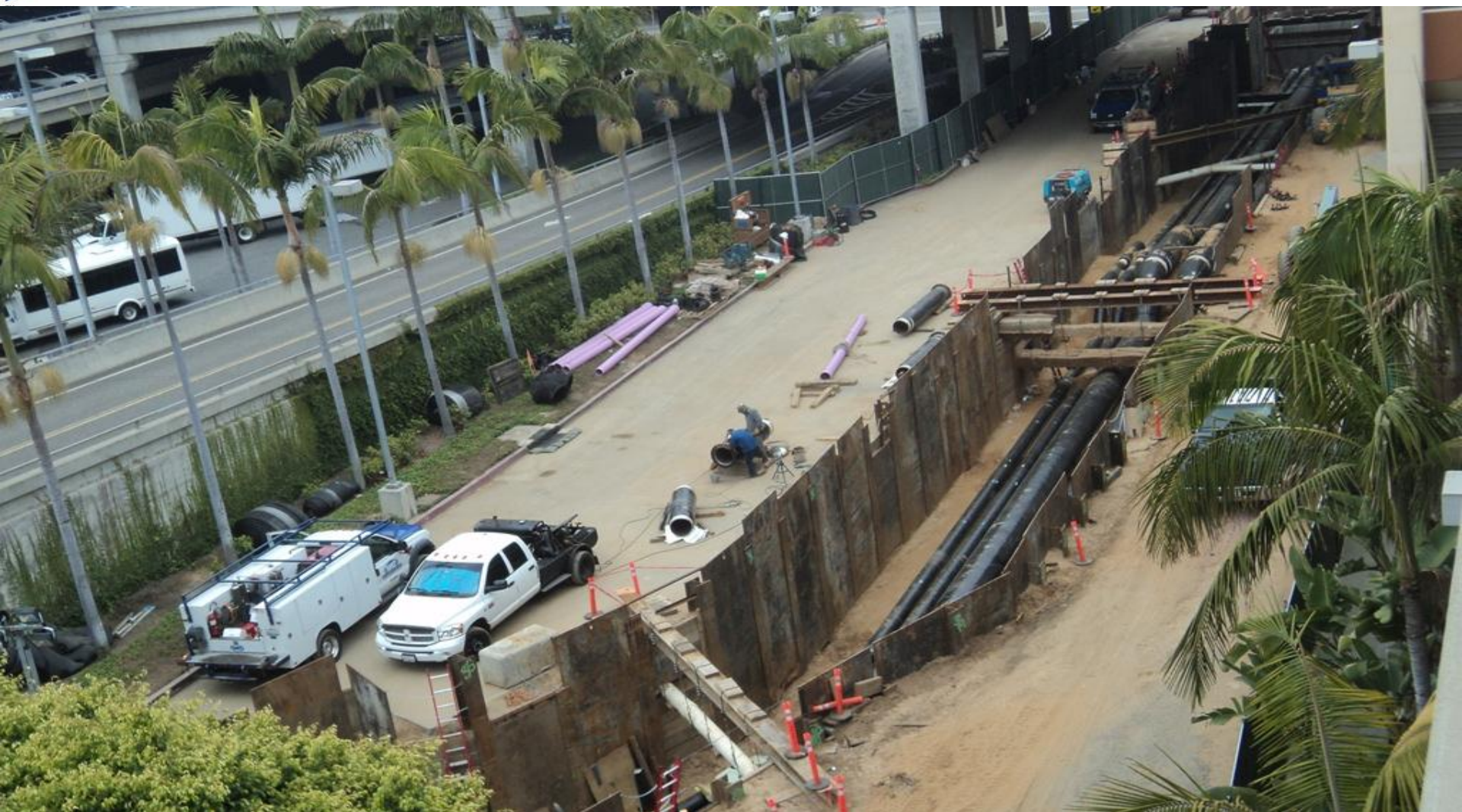
Utility distribution being installed along Center Way North. May 11, 2012
