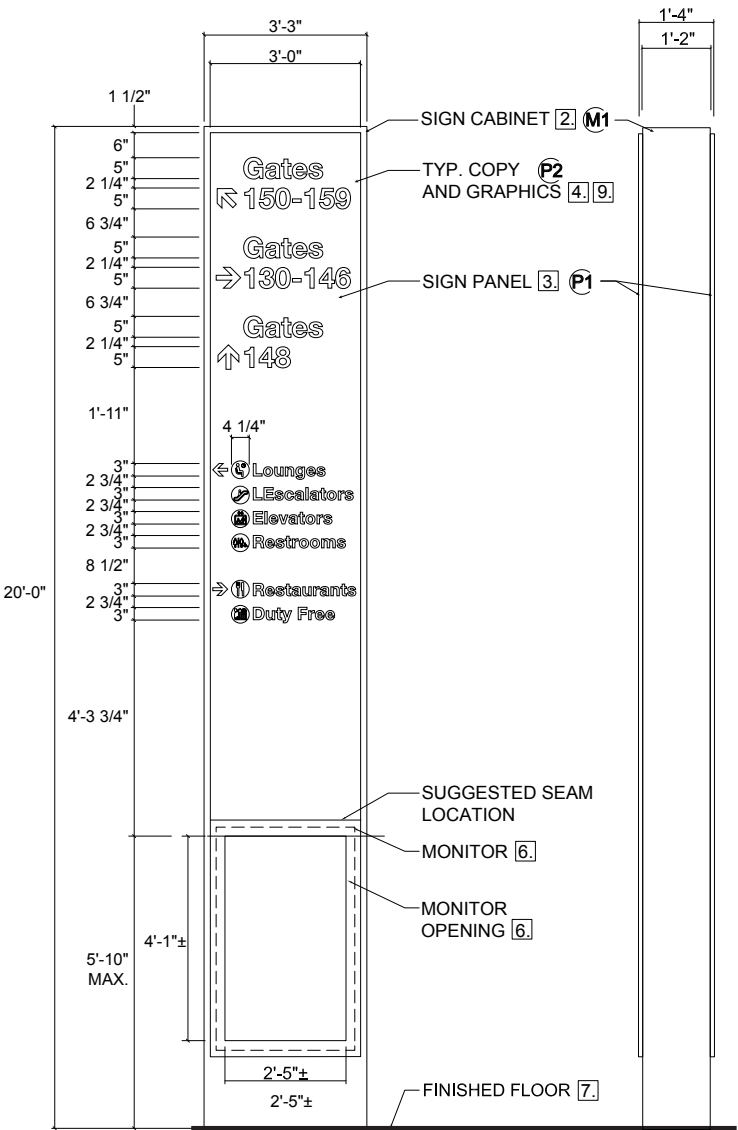
1 ELEVATION (SIDE A) NOT TO SCALE
