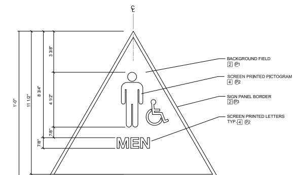
4 FRONT VIEW-MEN/WOMEN NOT TO SCALE
