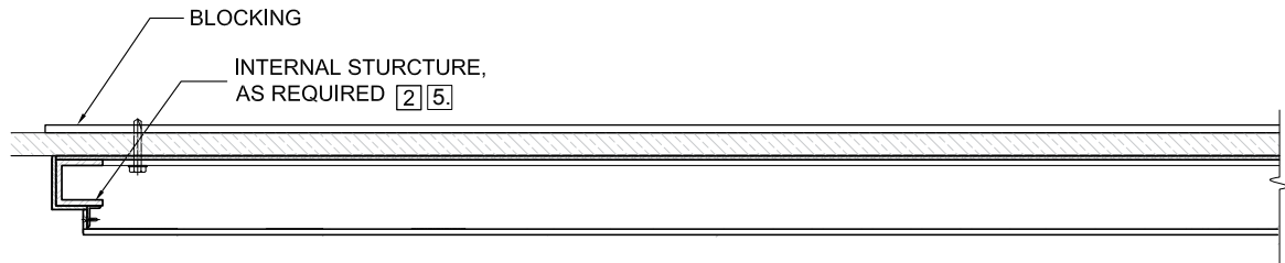
3 PARTIAL SECTION DETAIL NOT TO SCALE
