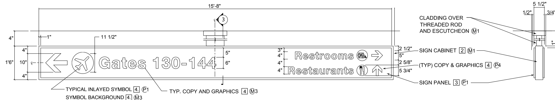
1 FRONT ELEVATION NOT TO SCALE
