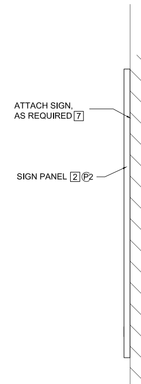
3 SIDE VIEW-MEN/WOMEN NOT TO SCALE
