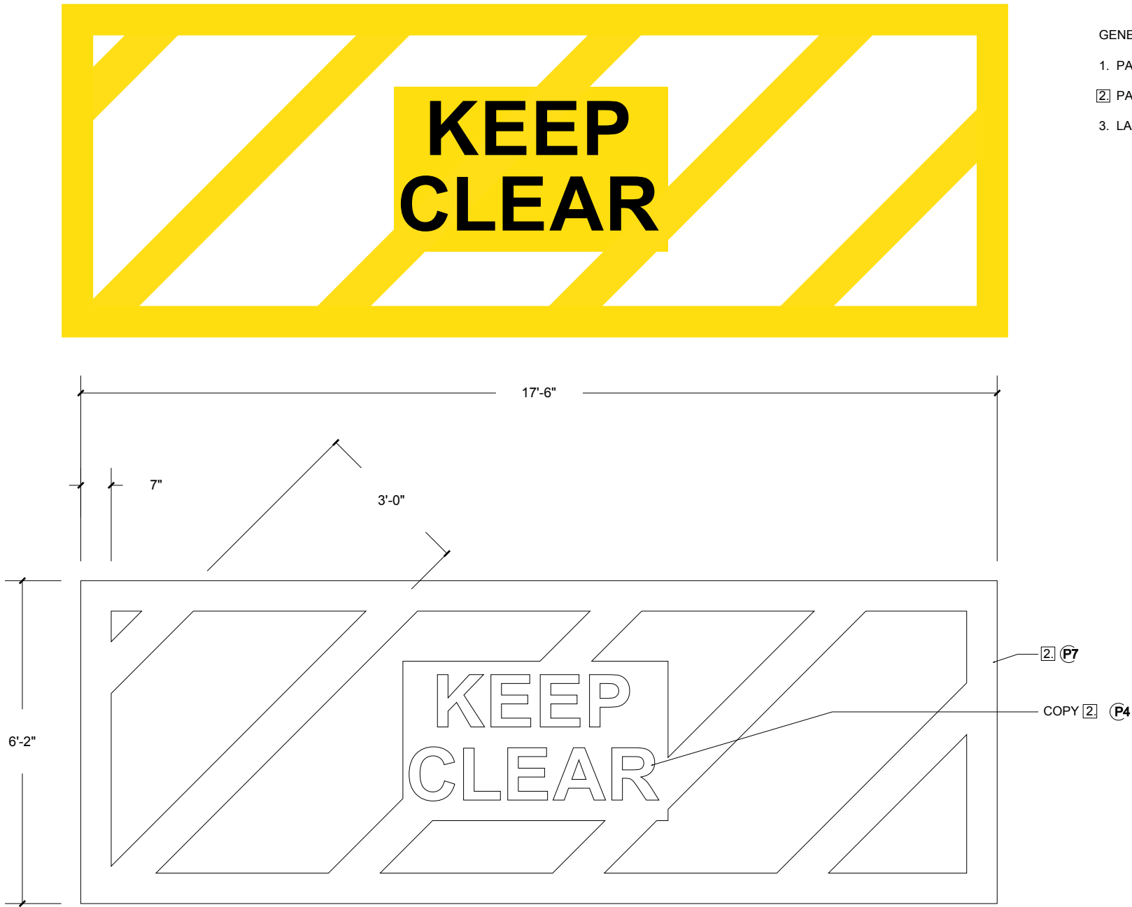
1 FRONT ELEVATION NOT TO SCALE
